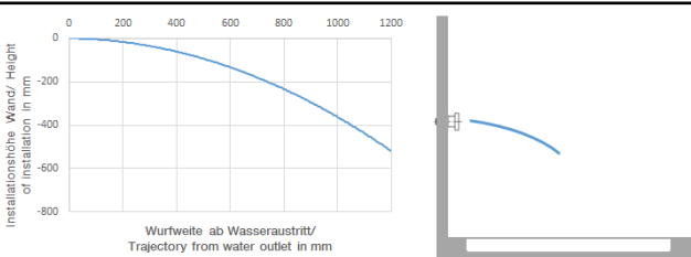
Trajectory diagram
